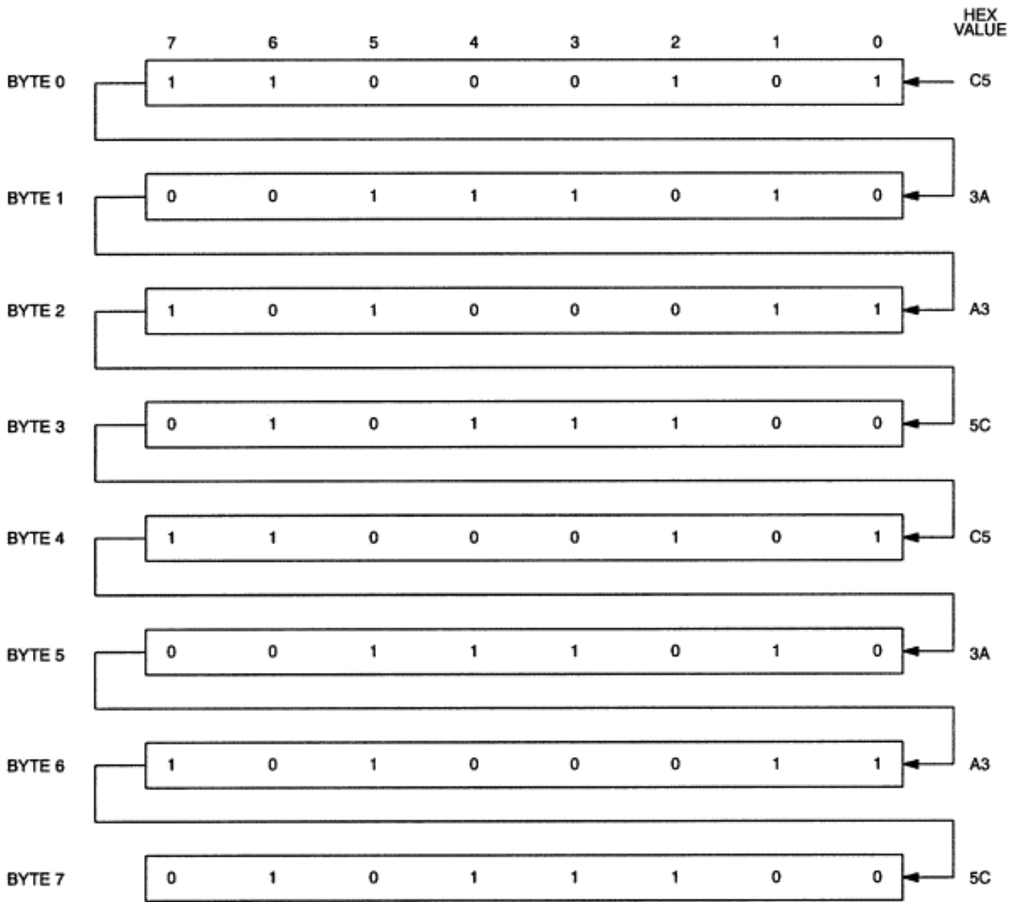
Figure 4. Time Chip Comparison Register Definition
