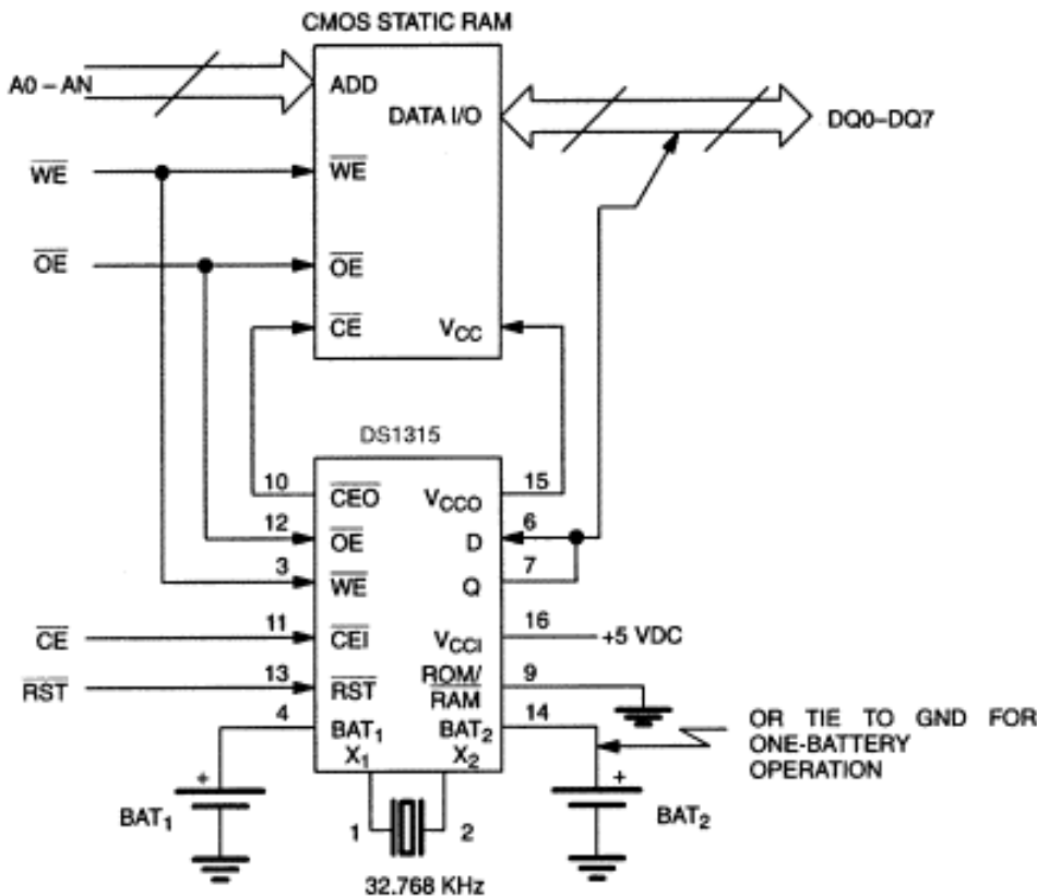
Figure 1. RAM/Time Chip Interface
