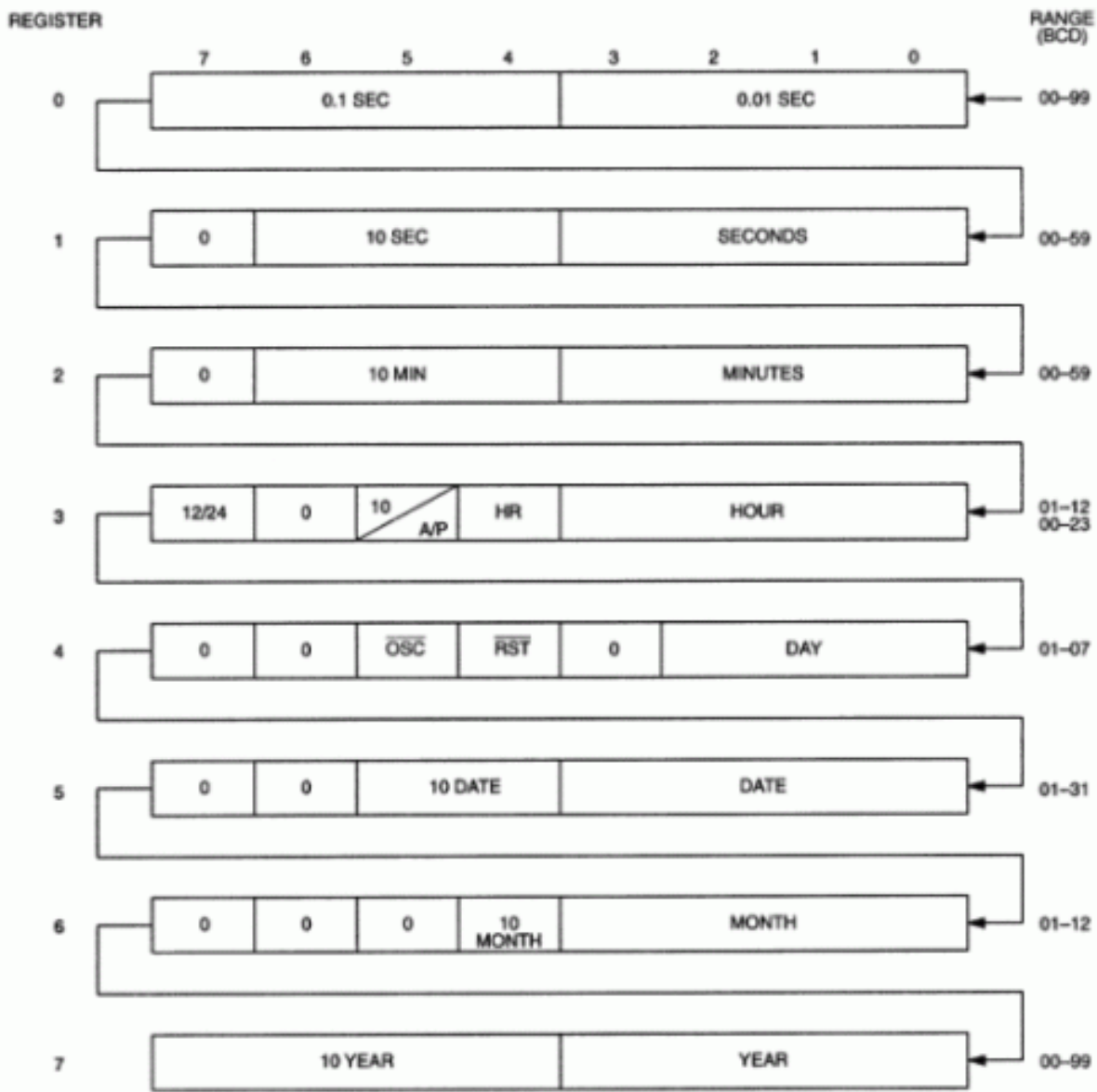
Figure 5. Time Chip Register Definition
