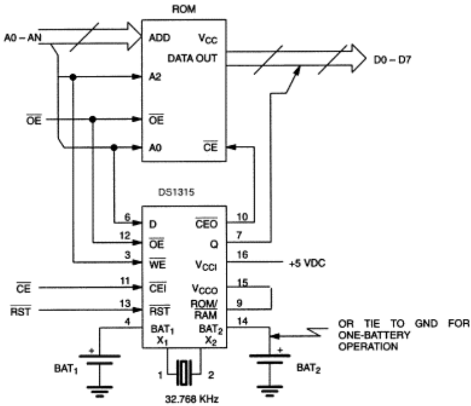
Figure 2. ROM/Time Chip Interface
