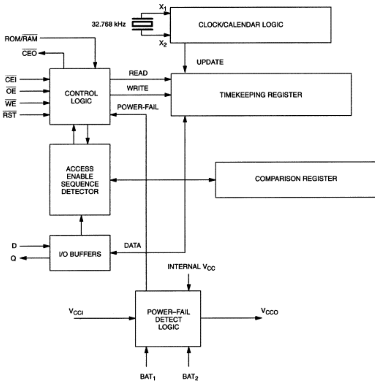
Figure 3. Timing Block Diagram
